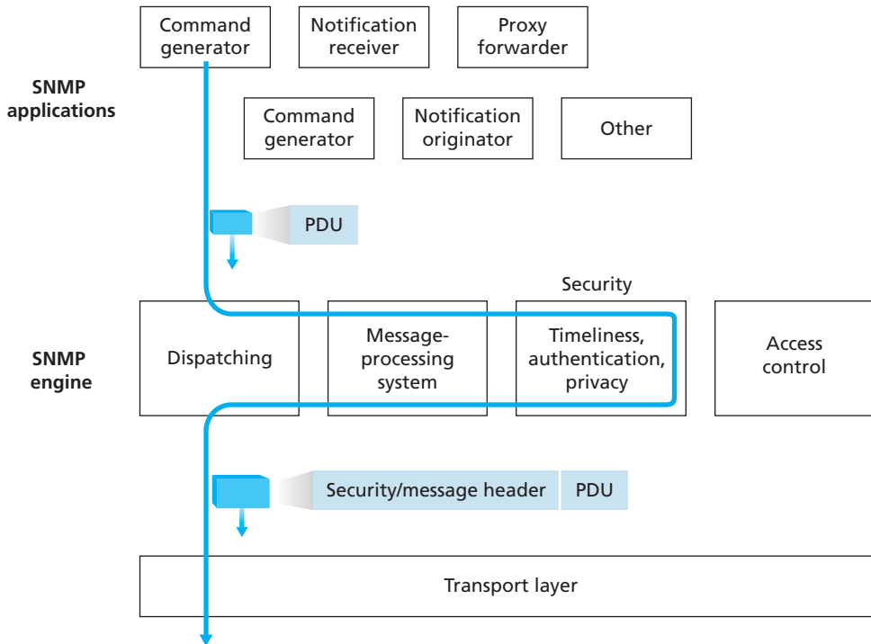
Figure 9.5 ♦ SNMPv3 engine and applications
