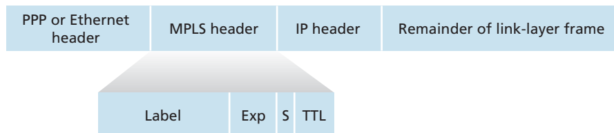
Figure 5.28 ♦ MPLS header: Located between link- and network-layer headers
